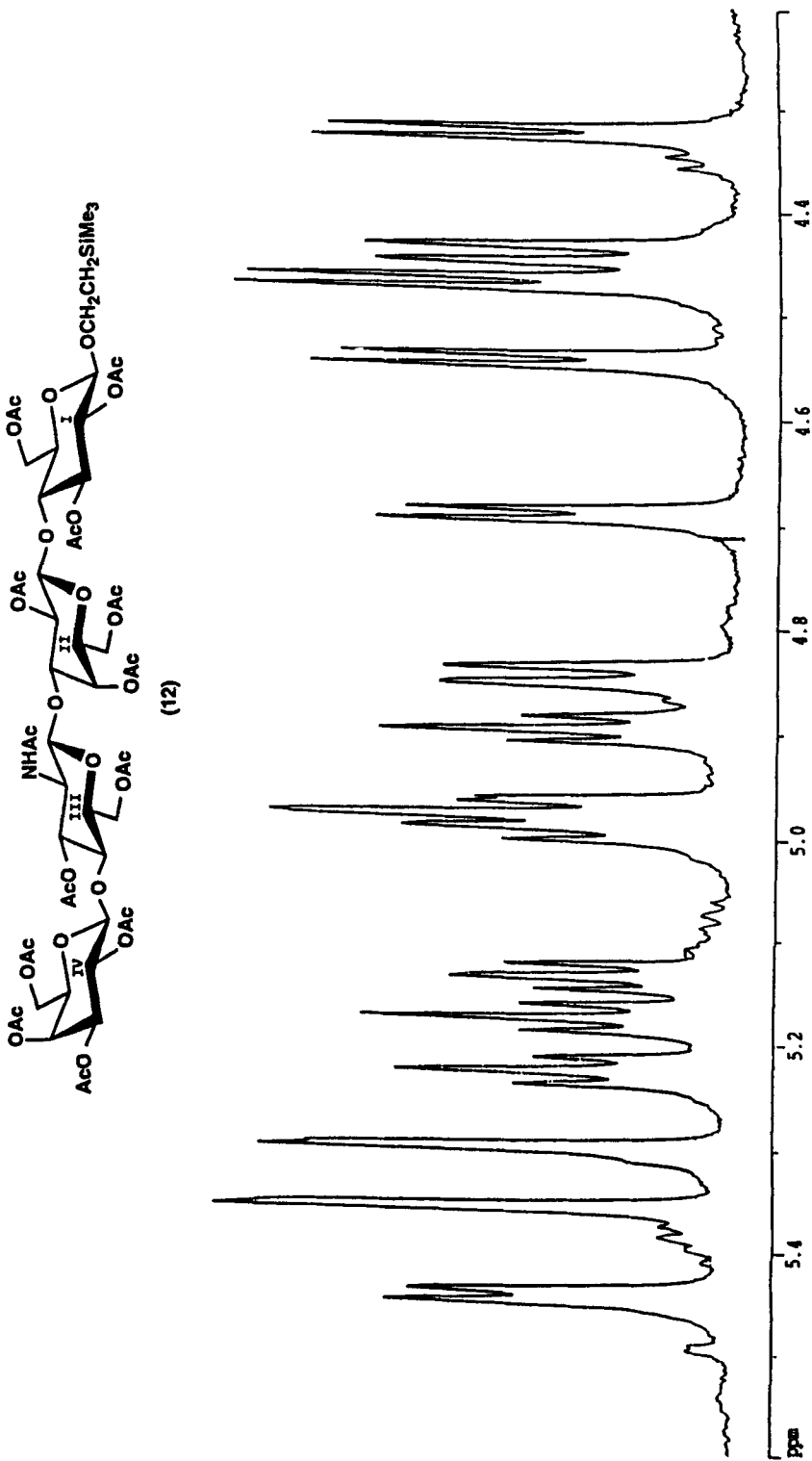
Figure 1. Partial proton ^1\text{H} NMR spectrum of the tetrasaccharide derivative 12 in \text{CDCl}_3 at 750 MHz.
